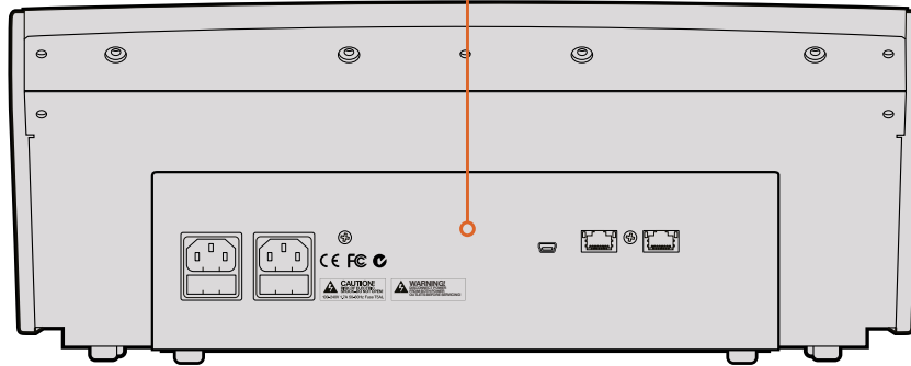
ATEM 1 M/E Broadcast Panel rear connectors
